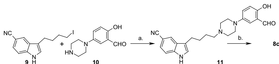
Scheme 5. Reagents and conditions: (a) acetonitrile, N -ethyl diisopropyl amine; (b) diethyl malonate, piperidine, glacial acetic acid.
