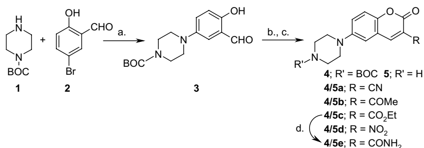
Scheme 1. Reagents and conditions: (a) Sodium tert -butylat; chloro-(di-2-norbornyl phosphino)-(2'-dimethyl-amino-1,1'-biphenyl-2-yl)-palladium(II), toluene; (b) malononitrile or RCH 2 CO 2 Et piperidine, acetic acid; (c) HCl, EtOH; (d) Pd/C, H 2 , EtOH; (d) (i) 25% NH 3 /water, (ii) HCl, EtOH.
