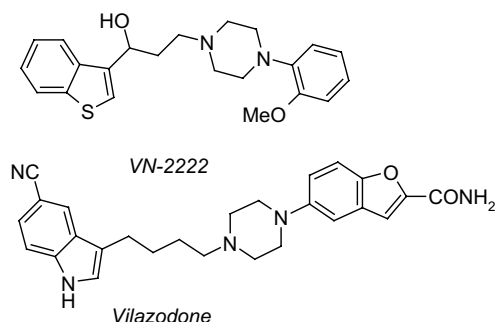
Chart 1. Dual 5-HT 1A ligands and 5-HT re-uptake inhibitors.
