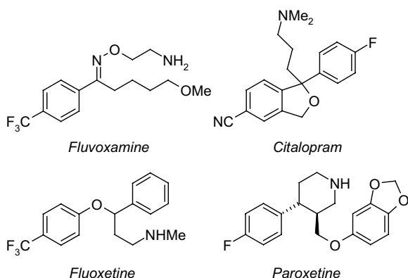
Chart 2. Established 5-HT re-uptake inhibitors.
