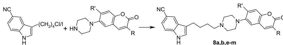
Scheme 4. A generic visualisation of the synthesis of compounds 8 .
