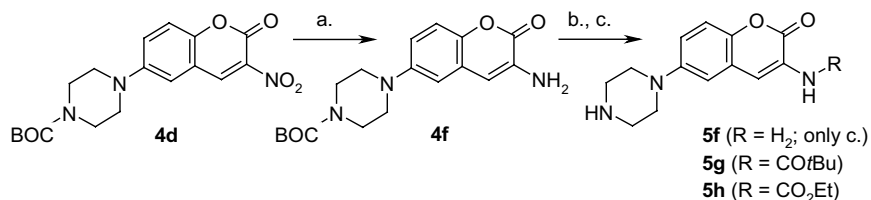
Scheme 2. Reagents and conditions: (a) 5% Pd/C, H 2 , EtOH; (b) RCOCl, base, dichloromethane; (c) HCl, EtOH.
