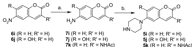
Scheme 3. Reagents and conditions: (a) Raney-Ni, H 2 , MeOH; (b) bis-(2-chloro ethyl)-ammonium chloride, NMP.
